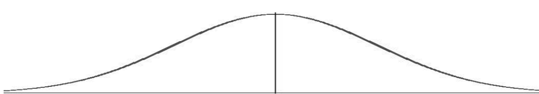
Fig. The bell curve is symmetrical
